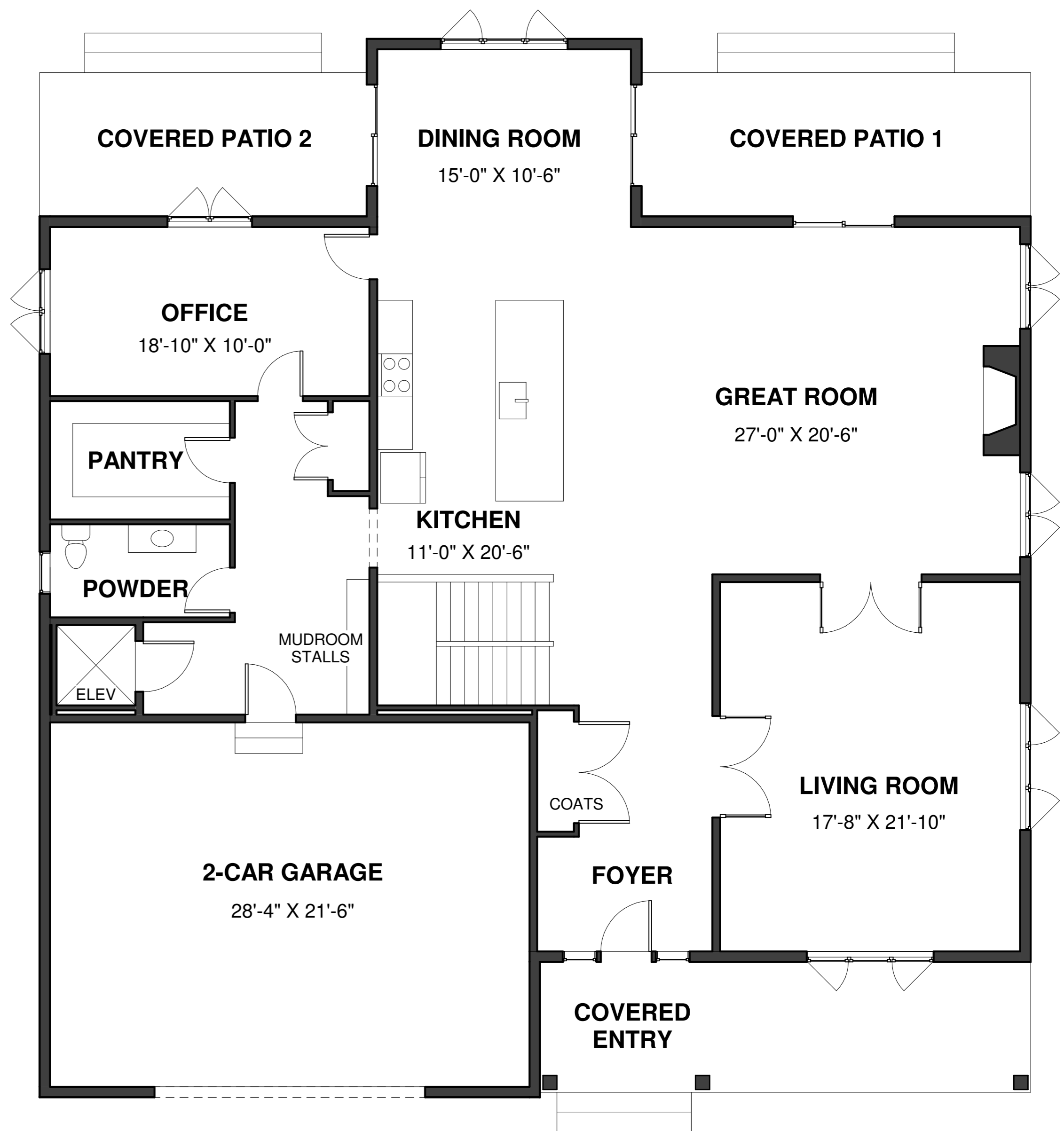
BASE DESIGN - FIRST FLOOR 10' CEILING HEIGHT 2,210 SF
