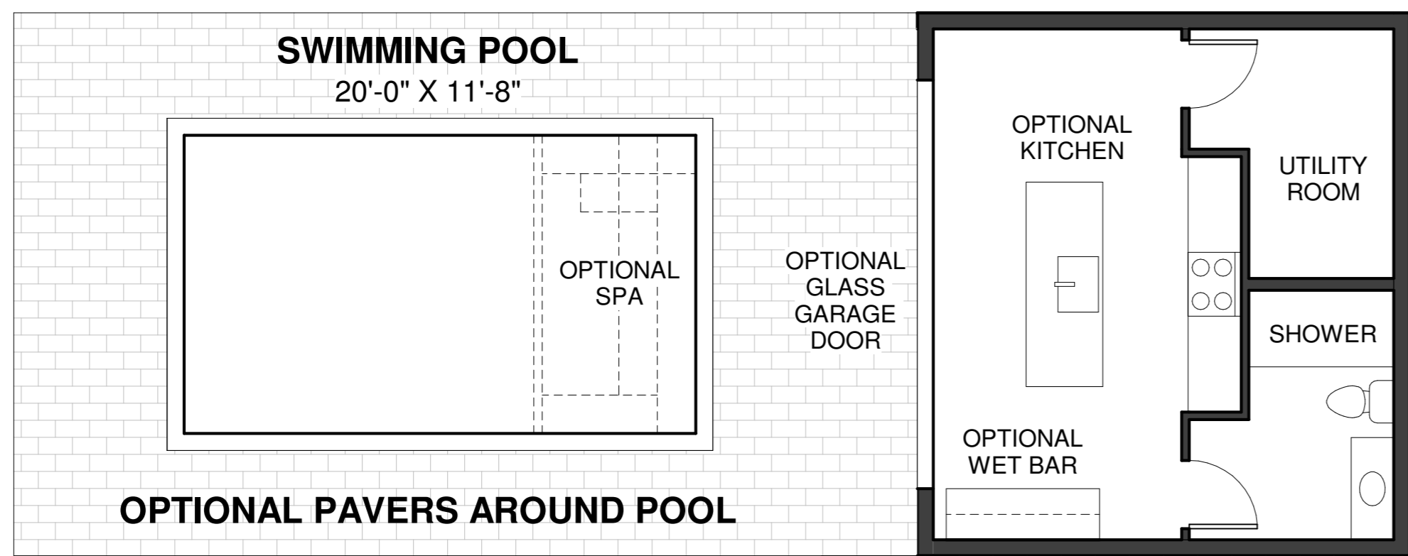
OPTIONAL POOL HOUSE 18'-0" X 20'-0"
