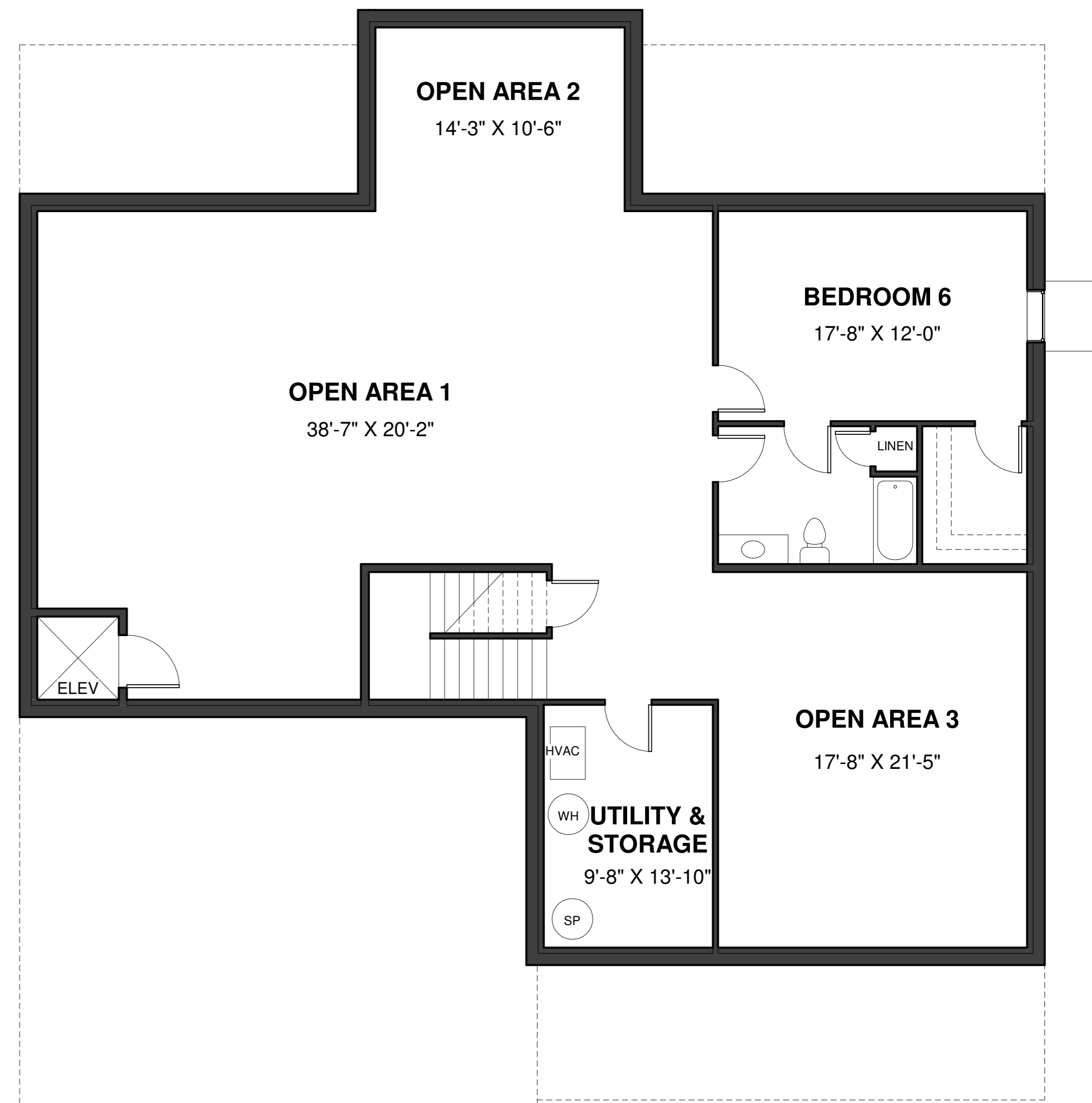
BASE DESIGN - BASEMENT FLOOR
