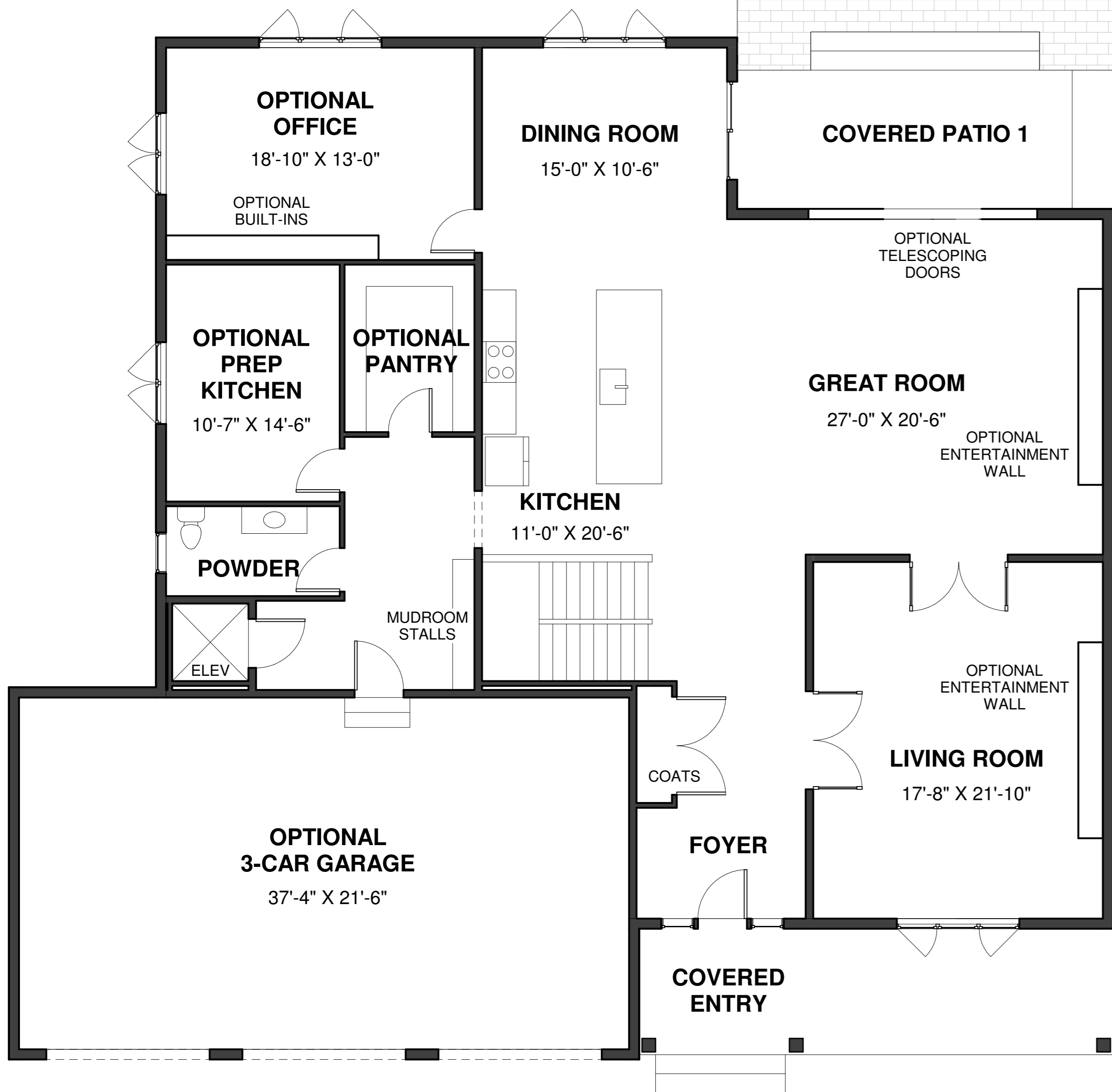
DESIGN OPTIONS - FIRST FLOOR 10' CEILING HEIGHT 2,413 SF
